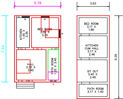
PROPOSED GROUND FLOOR PLAN
