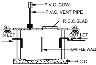
SEC. OF SEPTIC TANK
