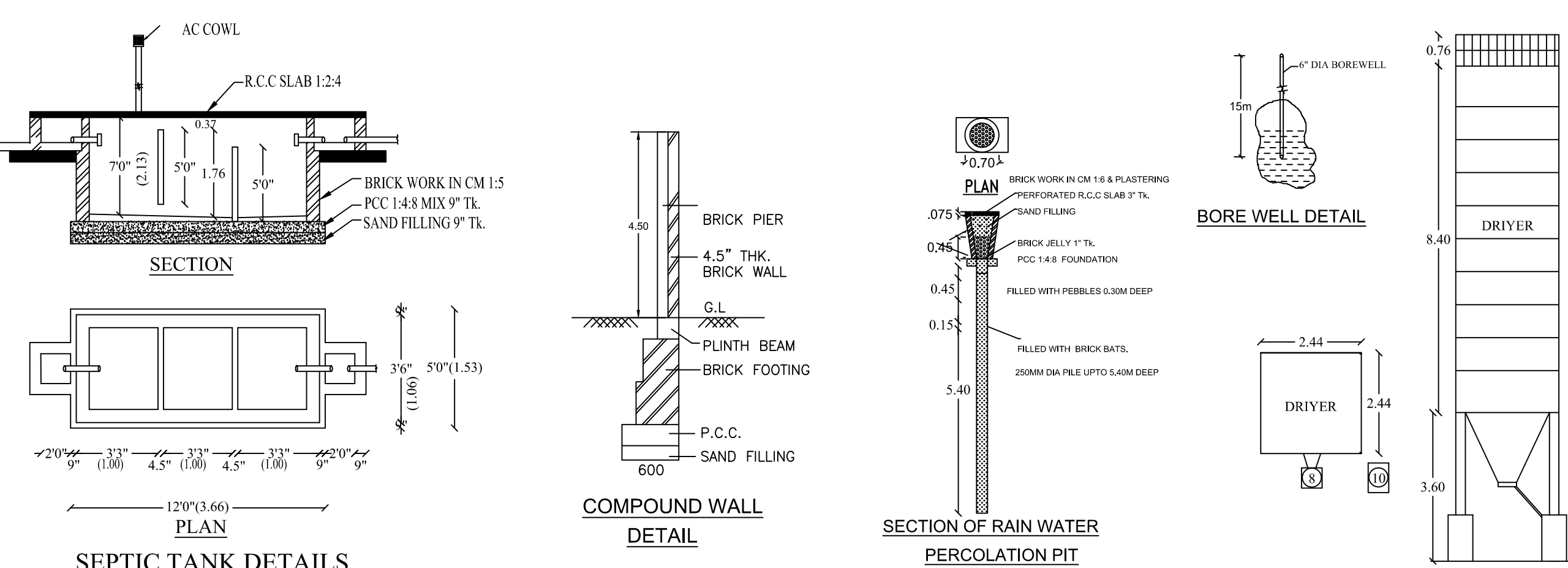
SEPTIC TANK DETAILS
