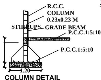
COLUMN DETAIL
