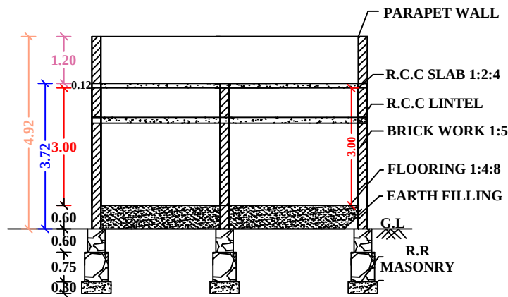
"SECTION "AB"
