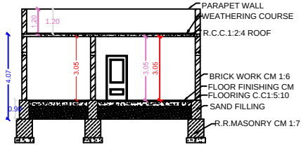
SECTION ON SV
