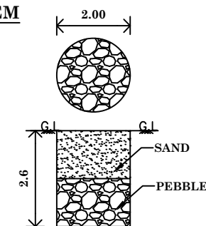
RAINWATER HARVESTING
