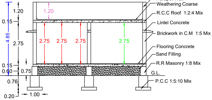
SECTION ON SS
