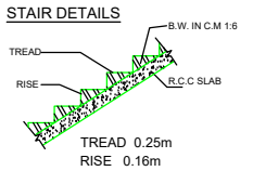
STAIR DETAILS
