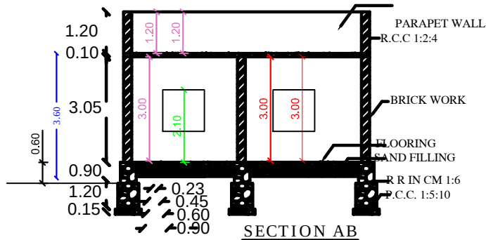
SECTION AB
