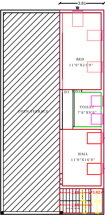
PRO.FIRST FLOOR PLAN
