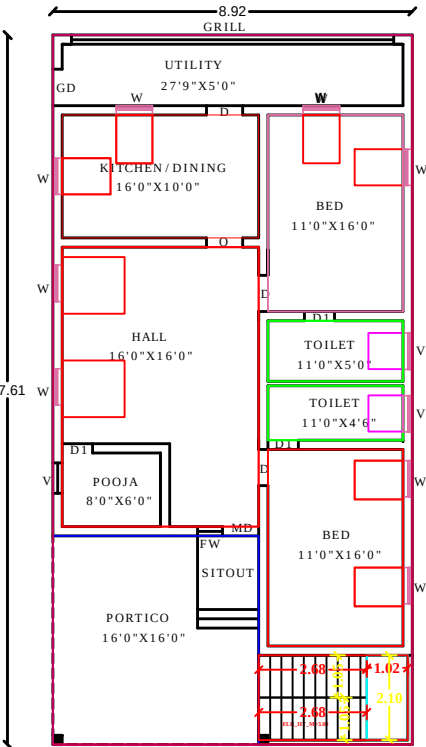
EXG.GROUND FLOOR PLAN
