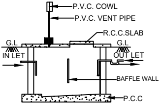
SEC. OF SEPTIC TANK
