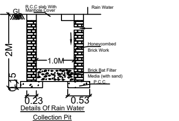
Details Of Rain Water Collection Pit (Recharge Well Method) SCALE:- 1"=4'0"
