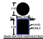
RAIN WATER HARVESTING
