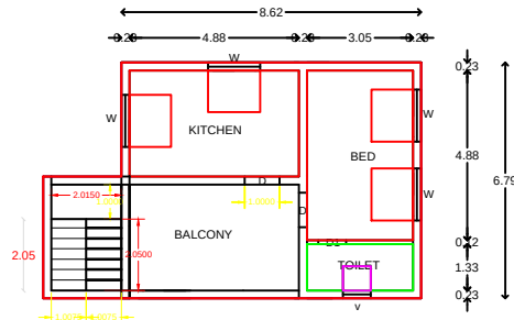
(PRO)F.FLOOR PLAN
