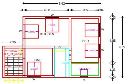
(EXD)G.FLOOR PLAN
