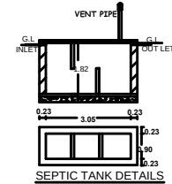
SEPTIC TANK DETAILS
