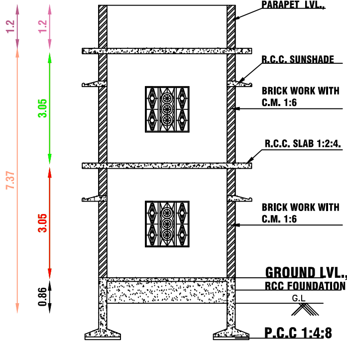
SECTION ON A-A & A'-A'
