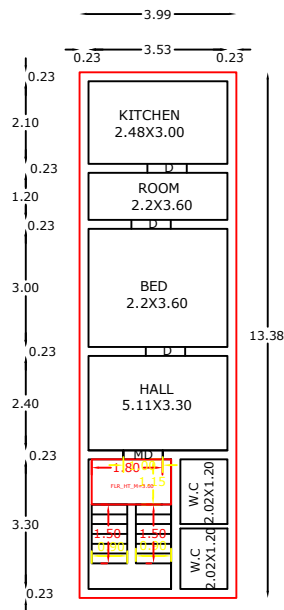
EXT GROUND FLOOR RESIDENTIAL PLAN
