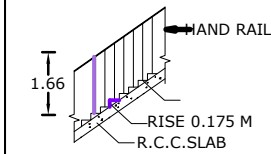
STAIRCASE
