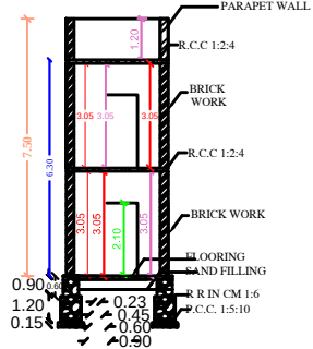
SECTION AB
