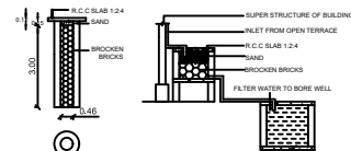
PERCOLATION PIT DETAILS OF FILTER BED & WELL
