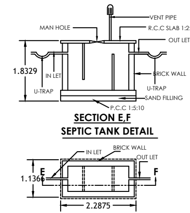
PLAN PLAN OF SEPTIC TANK
