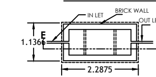
PLAN PLAN OF SEPTIC TANK
