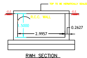
RWH SECTION
