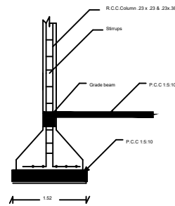
COLUMN DETAIL
