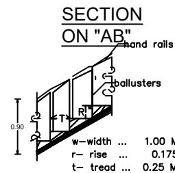
STAIR DETAILS
