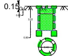
PERCOLATION PIT FOR 30 Sq.m (Scale:1:50)
