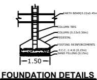
FOUNDATION DETAILS
