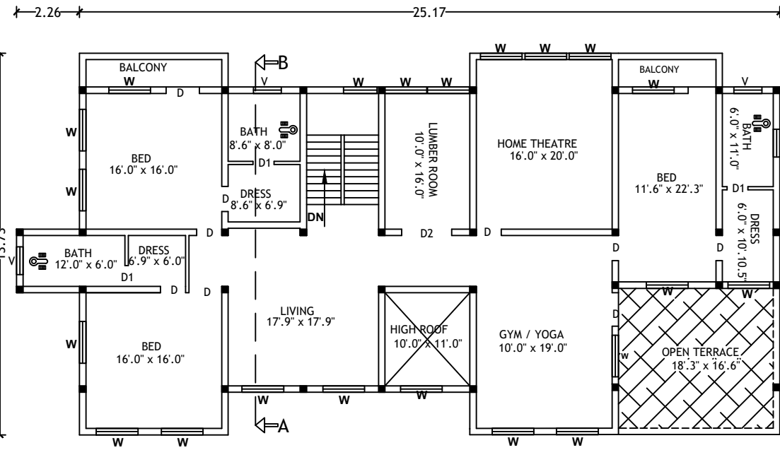
PLAN FIRST FLOOR
