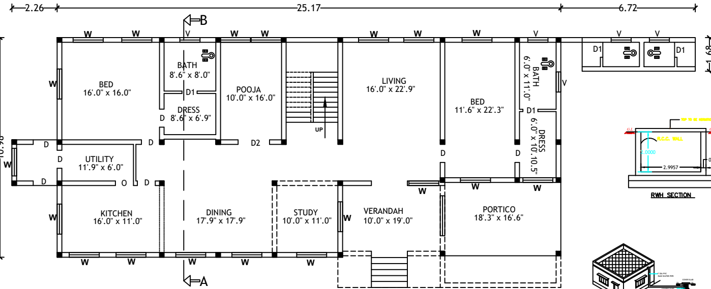
PLAN GROUND FLOOR
