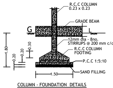
COLUMN - FOUNDATION DETAILS
