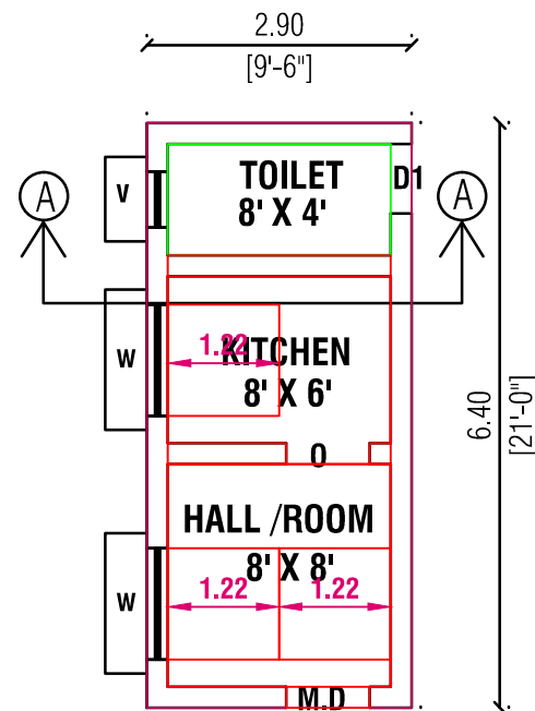
PLAN
