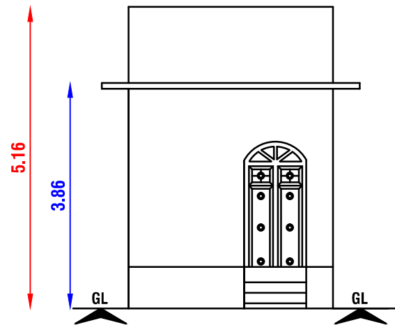
FRONT ELEVATION
