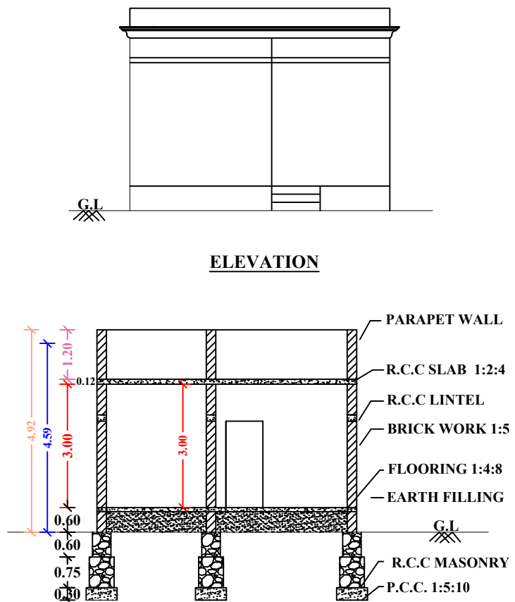
"SECTION "AB"
