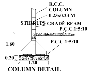
COLUMN DETAIL
