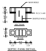
SEPTIC-TANK DETAIL
