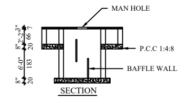
SEPTIC-TANK DETAIL
