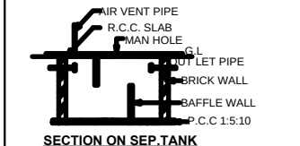
SECTION ON SEP.TANK
