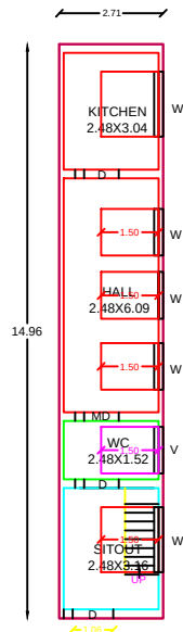
GROUND FLOOR PLAN
