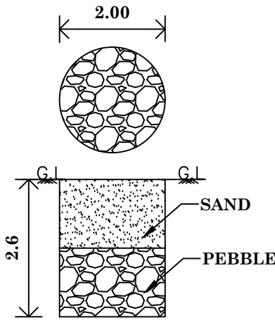
RAINWATER HARVESTING
