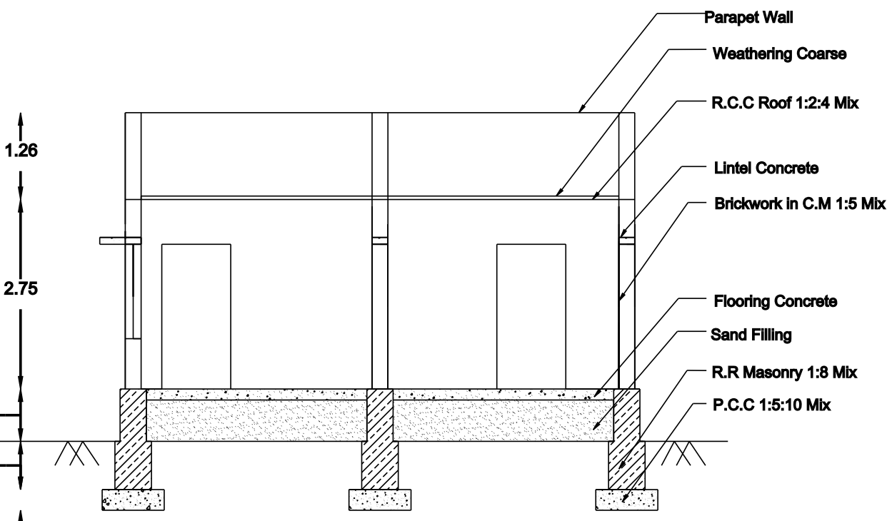
SECTION ON SS
