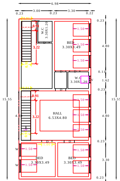
FIRST FLOOR RESIDENTIAL PLAN
