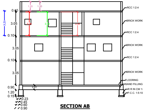
SECTION AB
