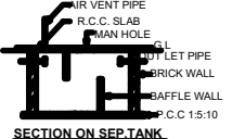
SECTION ON SEP.TANK
