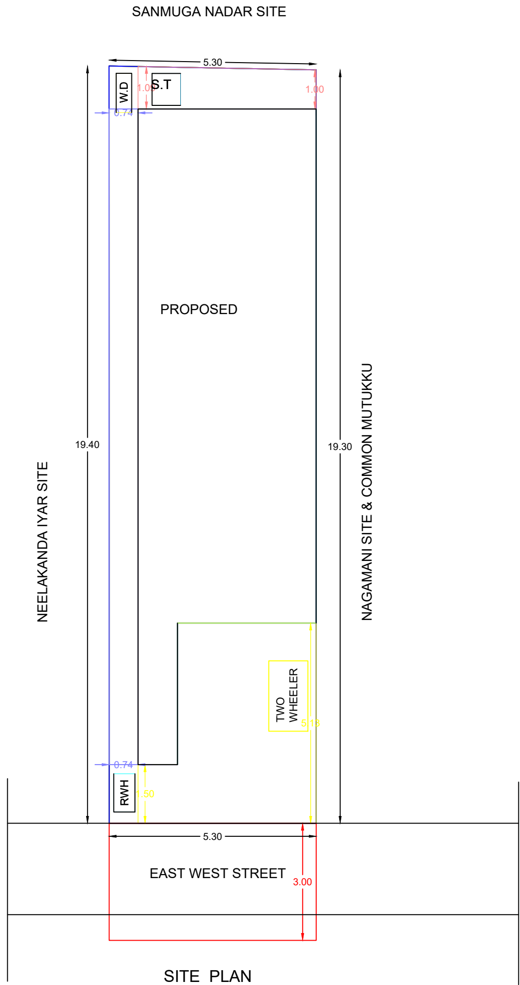
SITE PLAN
