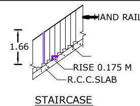
STAIRCASE
