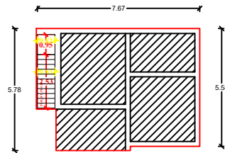
EXG.GROUND FLOOR PLAN
