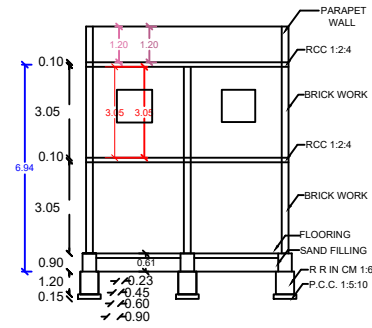
SECTION AB
