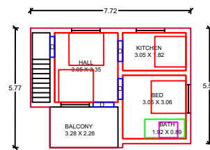
PRO.FIRST FLOOR PLAN
