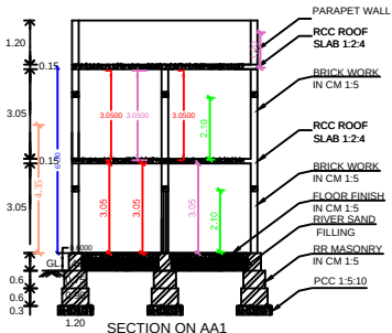
SECTION ON AA1
