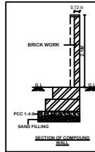
SECTION OF COMPOUND WALL
