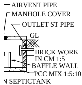
SECTION ON SEPTICTANK
