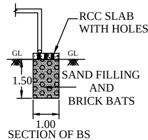
SECTION OF BS
