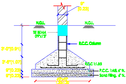
FOUNDATION DETAIL
