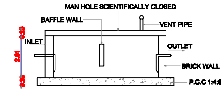
SECTION OF SEPTIC TANK
