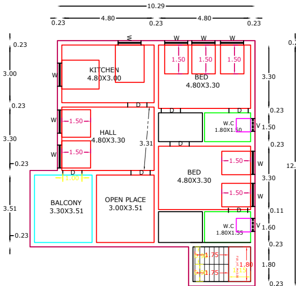
PRO FIRST FLOOR RESIDENTIAL PLAN
