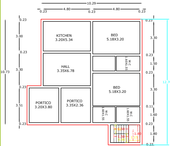
EXT GROUND FLOOR RESIDENTIAL PLAN
