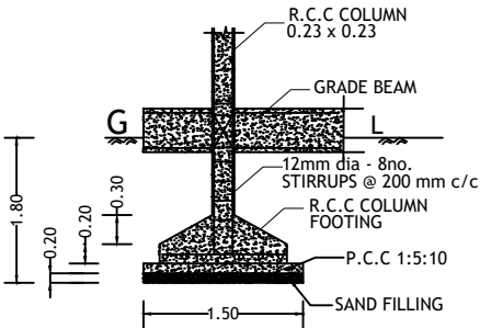
COLUMN - FOUNDATION DETAILS
