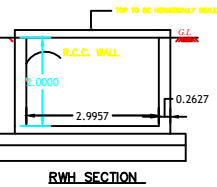
RWH SECTION
