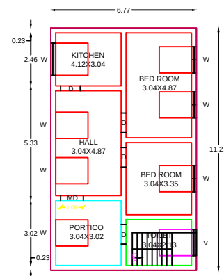
PROPOSED G.FLOOR
