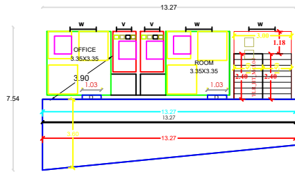
GROUND FLOOR PALN
