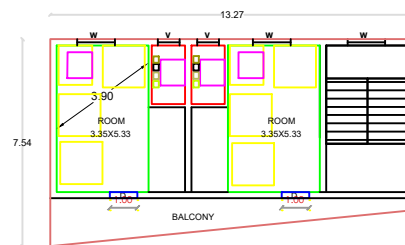
FIRST FLOOR PALN
