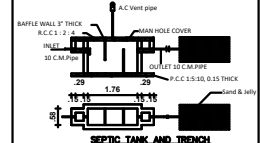
SEPTIC TANK AND TRENCH
