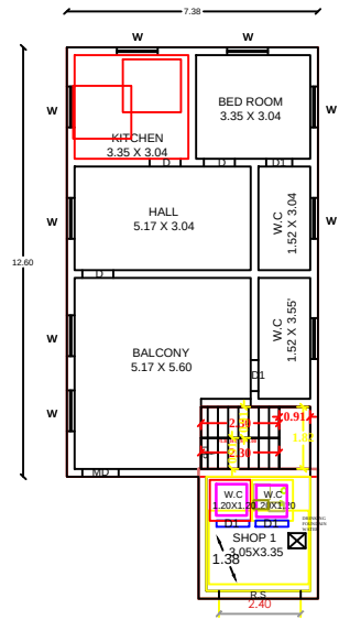
EXISTING G.FLOOR PROPOSED SHOP BUILDING
