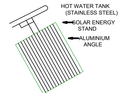
DETAILS OF SOLAR WATER HEATER
