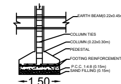
FOUNDATION DETAILS
