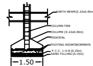
FOUNDATION DETAILS
