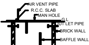
SECTION ON SEP.TANK
