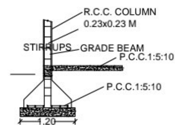
COLUMN DETAIL
