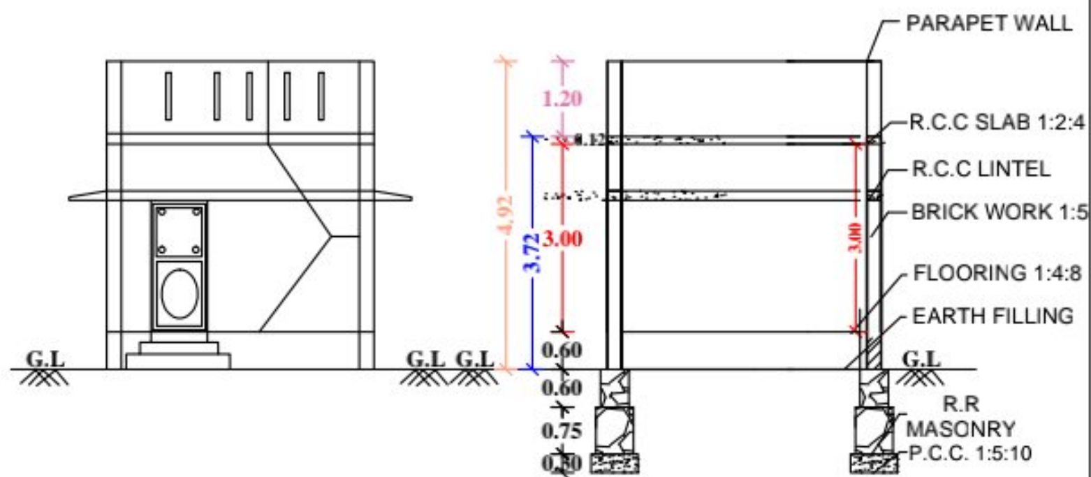
FRONT ELEVATION
