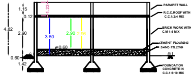
SECTION ON "AB"
