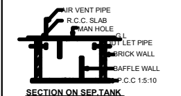
SECTION ON SEP.TANK
