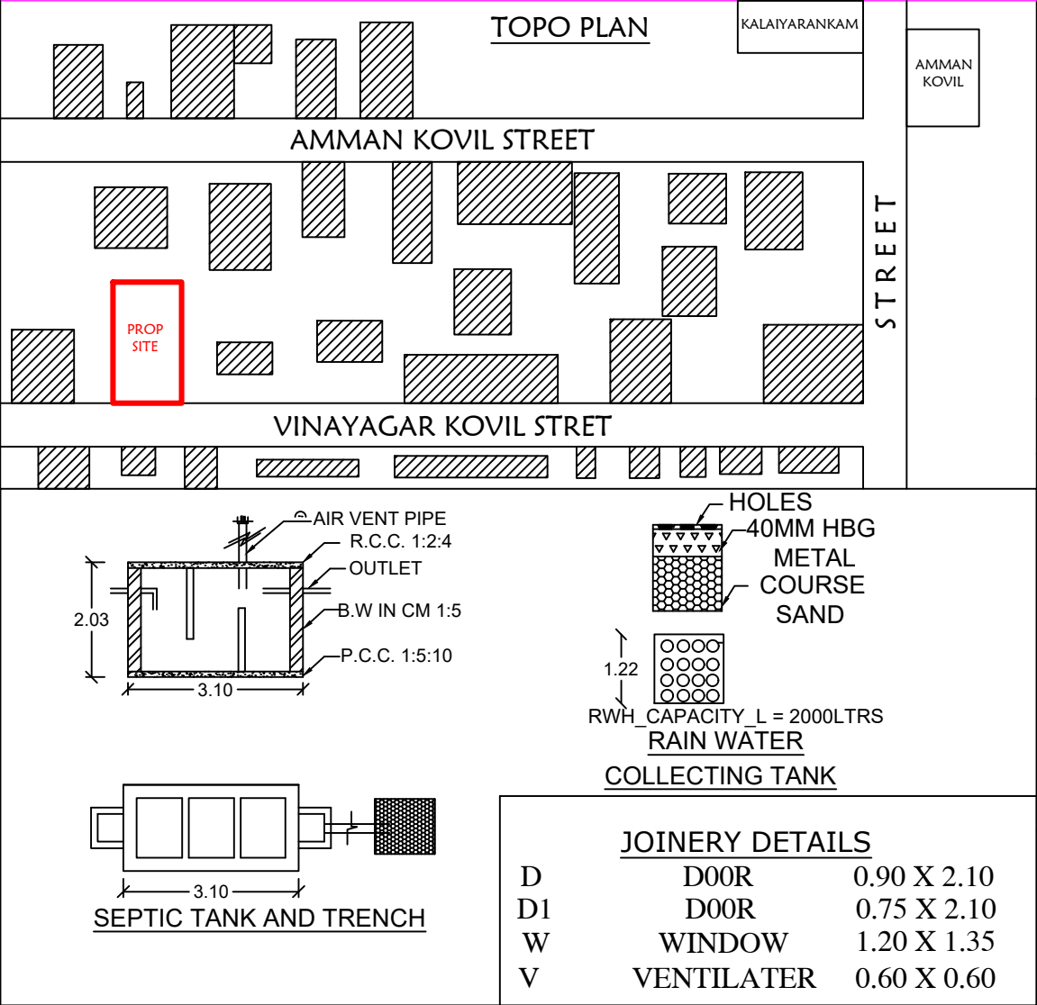
SITE PLAN
