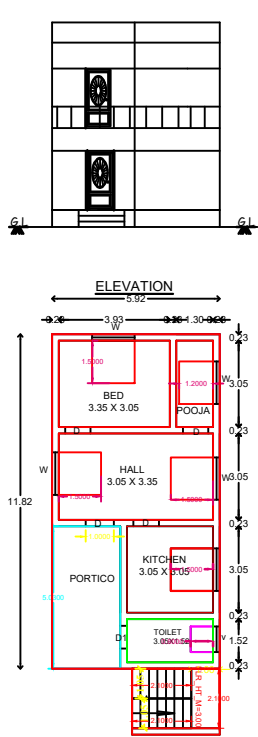
(EX)G.FLOOR PLAN
